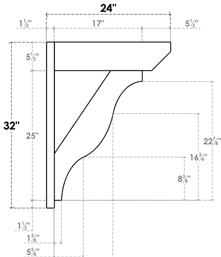
SIDE PROFILE
